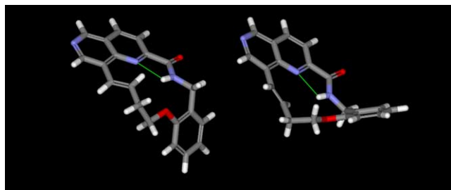
Figure 3. Crystal structure of macrocycle 2 .
