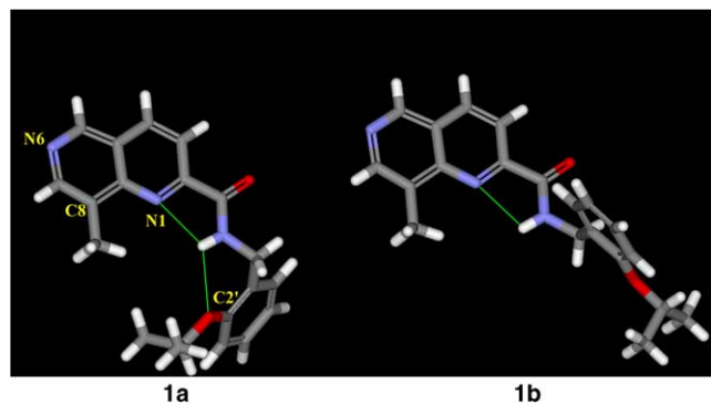
Figure 1. Crystal structure of 1 .
