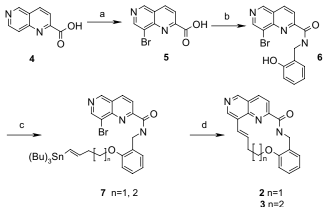
Scheme 1. Reagents and conditions: (a) AcOH, Br 2 , 80%; (b) HOBt, EDCI, 2-hydroxy-benzylamine, Et 3 N, DMF, 93%; (c) ( n = 1) DEAD, 4-tributylstannanyl-but-3-en-1-ol, Et 3 N, DMF (53%); ( n = 2) DEAD, 4-tributylstannanyl-pent-3-en-1-ol, Et 3 N, DMF (50%); (d) Pd(dba) 3 ·CHCl 3 , DMF, 110 °C, 3 h. n = 1, 35%; n = 2, 28%.
